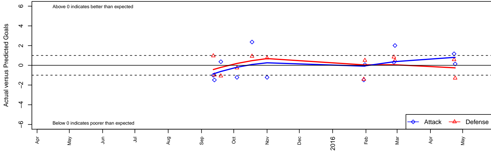
Real Colorado ECNL G00 Dots are actual minus expected GF (blue circles) and GA (red triangles). Blue line is smoothed change in attack strength. Red is smoothed change in defense strength.
